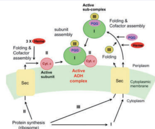
Molecular architecture of membrane-bound alcohol dehydrogenase in acetic acid bacteria
