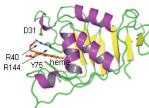
The Structure of Heme Acquisition System A from Y. pseudotuberculosis
