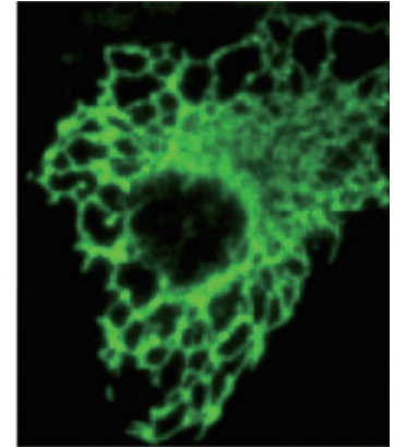
Discovery of an N-myristoylated transmembrane protein that induces endoplasmic reticulum (ER) morphological change
